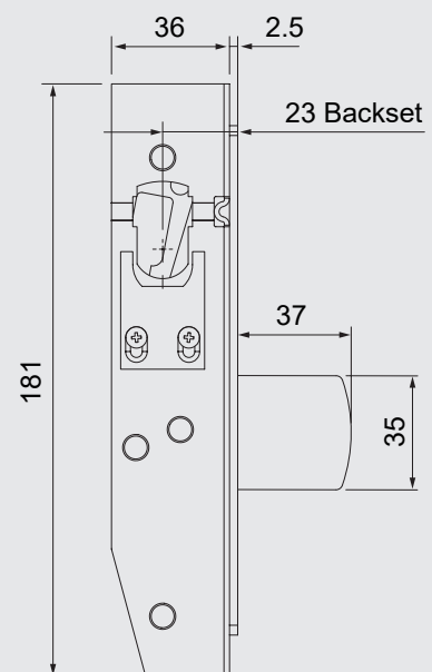
950-37 lock body
