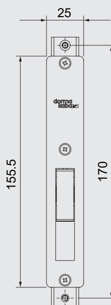
Face plate
