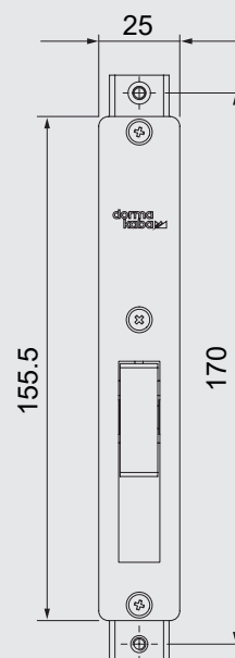
Face plate
