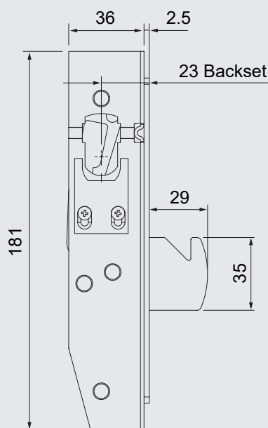
951 lock body
