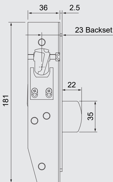
950-22 lock body
